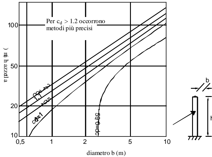
Fig. C.7.11 (c) - Ciminiere in c.a.
