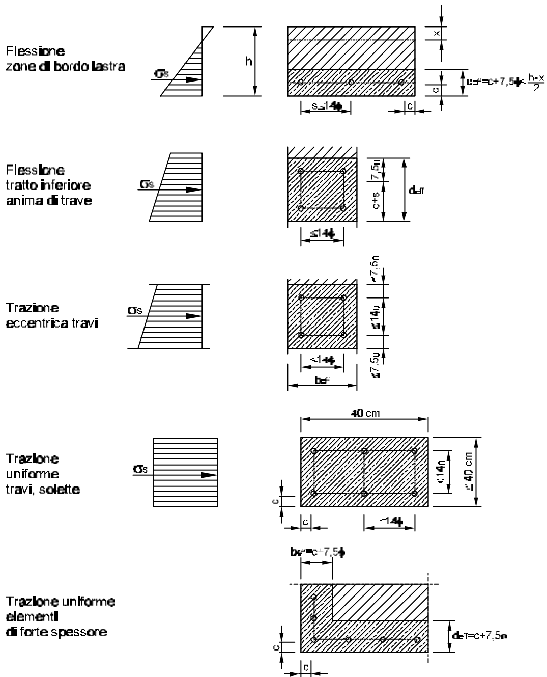
Fig. 4 - Area efficace
